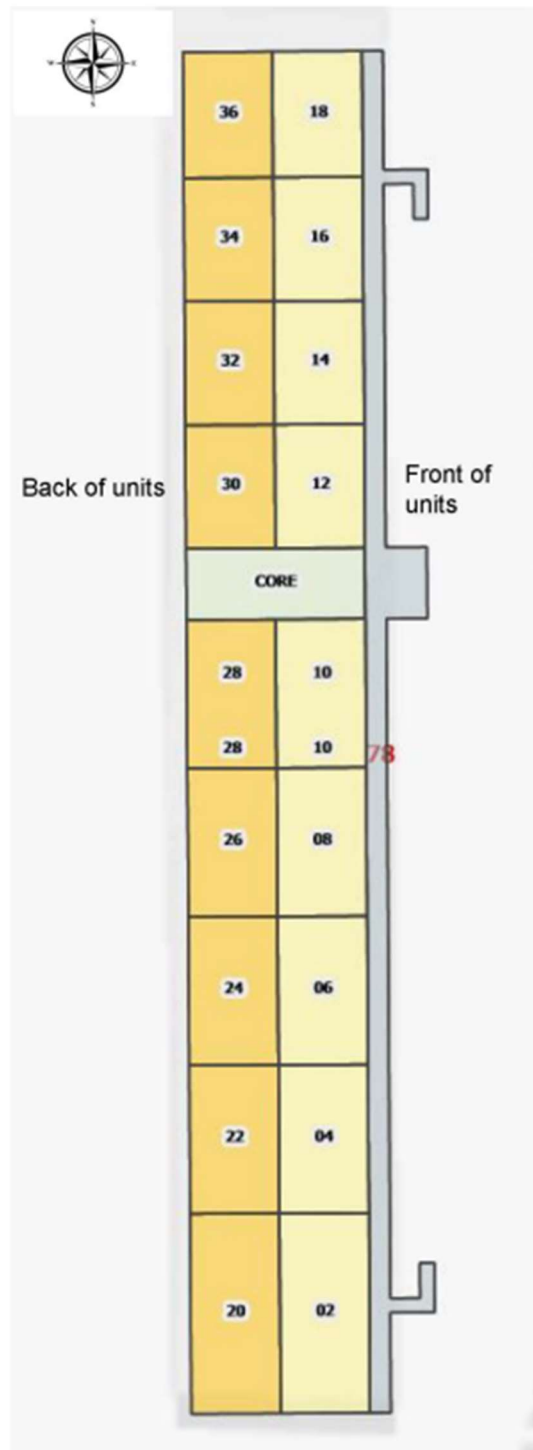
Figure 3. Plan view of subject building with unit layout.
